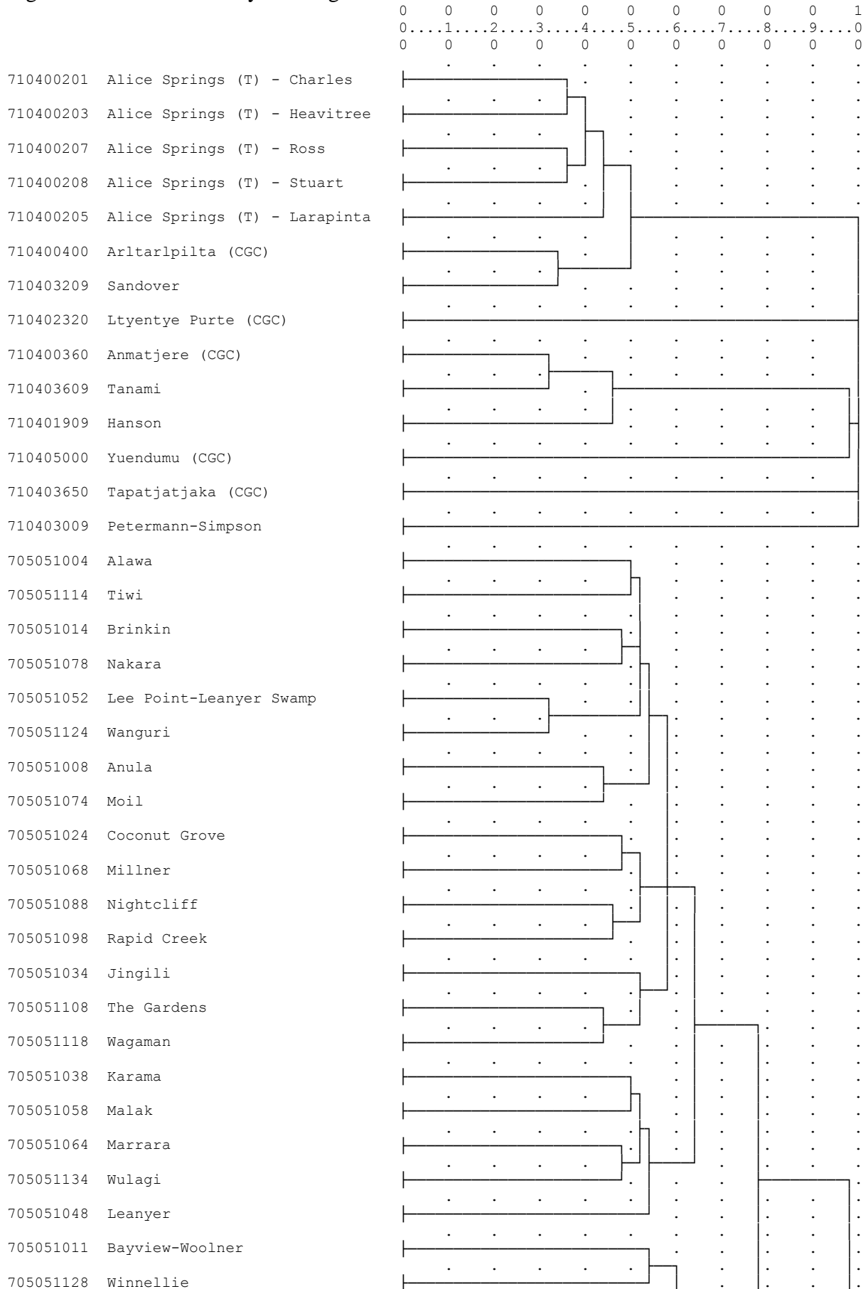
Figure 4 Northern Territory dendrogram minus Coomalie
